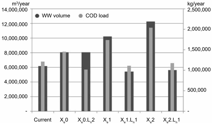
Figure 13.13. Changes in wastewater quantity and COD load under the six scenarios in the study area’s water drainage network in 2030
