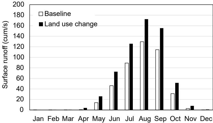
Figure 11.6. Comparison of surface runoff between baseline and increased deforestation scenario for the Lower Monywa sub-basin
