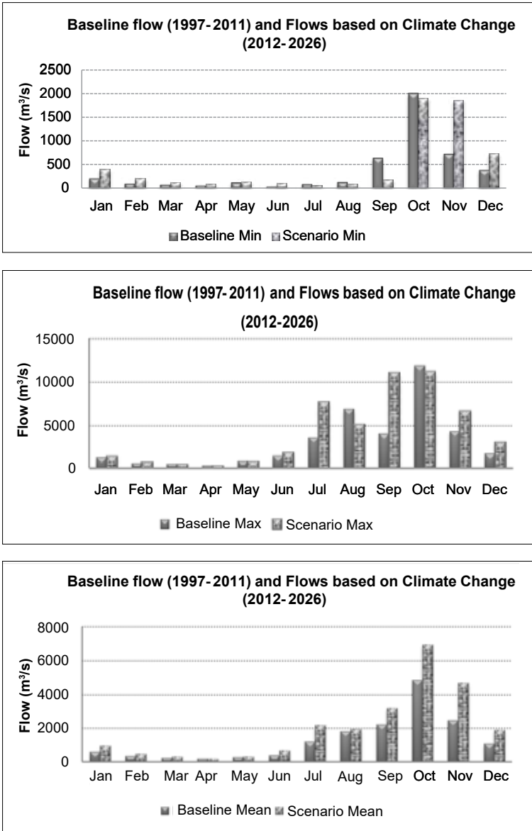
Figure 10.4. Variations in monthly flow at sub-catchment 3 (Peam Kley Station) due to climate change scenario (2012 to 2026) compared to the baseline monthly flow (1997–2011) under maximum, minimum and average conditions
