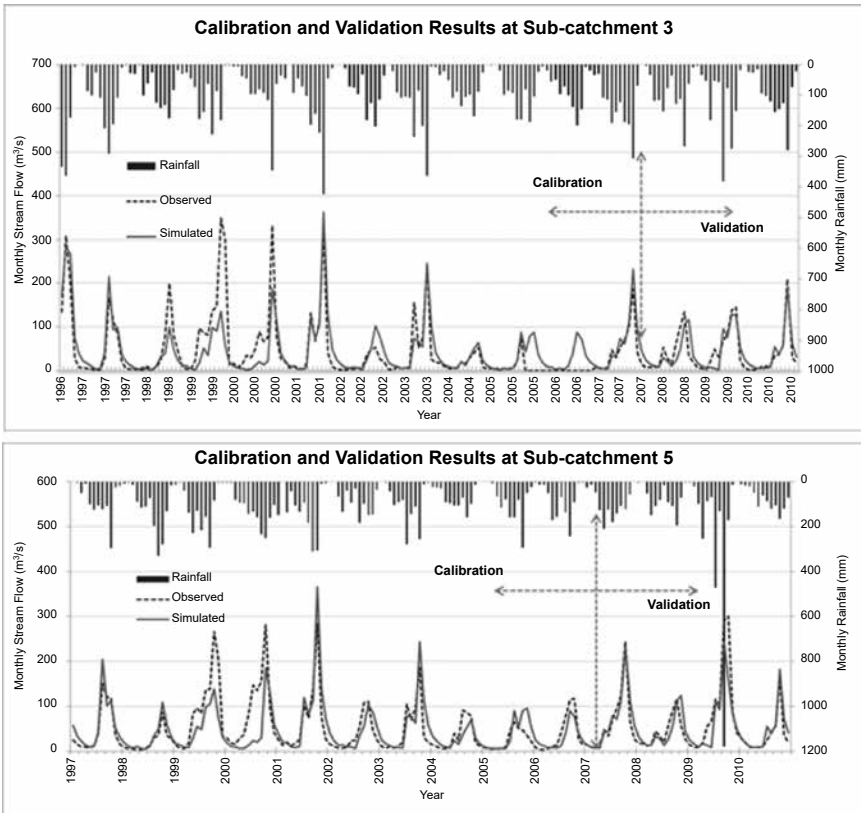
Figure 10.3. Simulated baseline flows from 1996 to 2011 at sub-catchments 3 and 5
