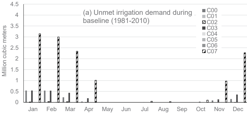
Figure 12.7. Unmet water demand for irrigation sector during (a) baseline and (b) future dry climate conditions at the sub-basin level
