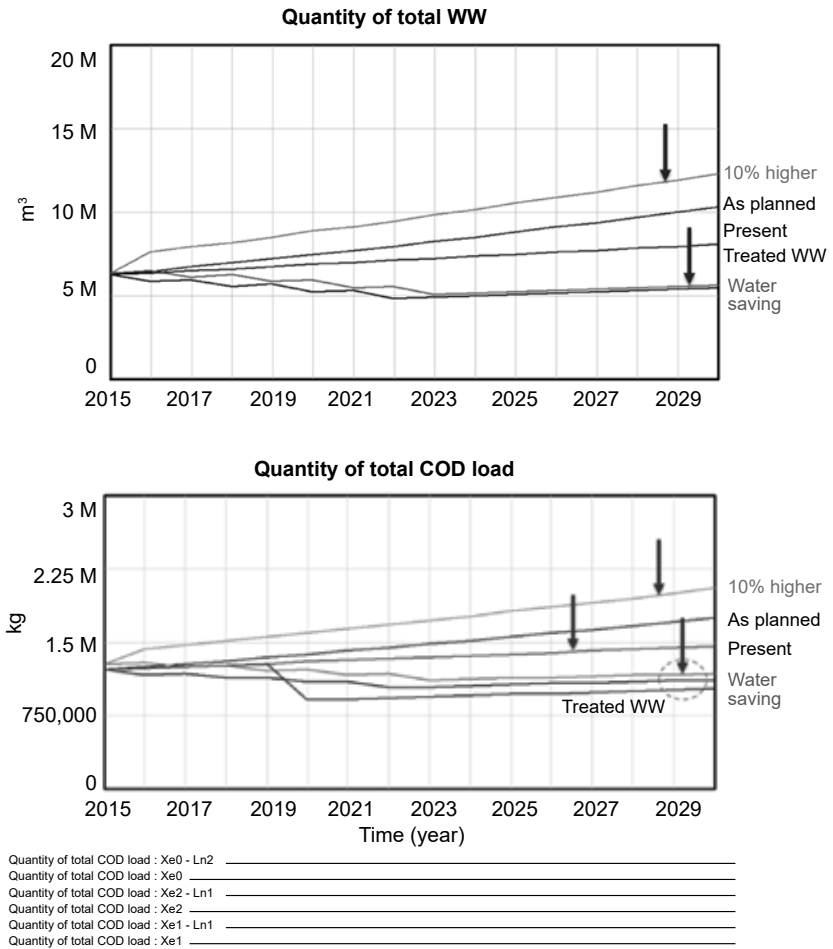
Figure 13.12. Changes in wastewater (WW) quantity and COD load under the six scenarios in the study area's water drainage network from present to 2030
