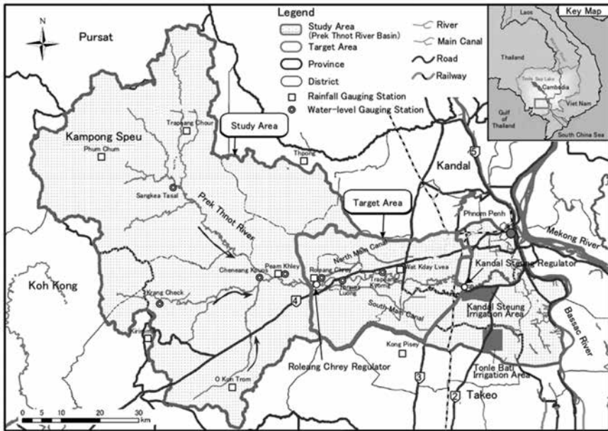
Figure 10.1. Project study area, Prek Thnot River Basin
