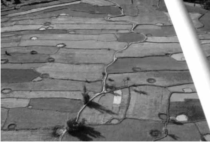
Figure 3.6. Bomb craters from the Vietnam War located in paddies of southern Lao PDR. Note the uniform appearance of perimeters of each crater. Photo taken on August 16, 1996 by Jeb Barzen.
