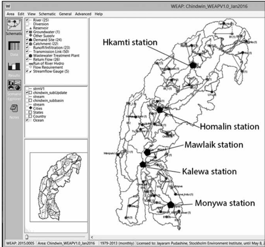
Figure 11.3. Schematic of the WEAP model for the Chindwin River Basin and discharge stations for model calibration
