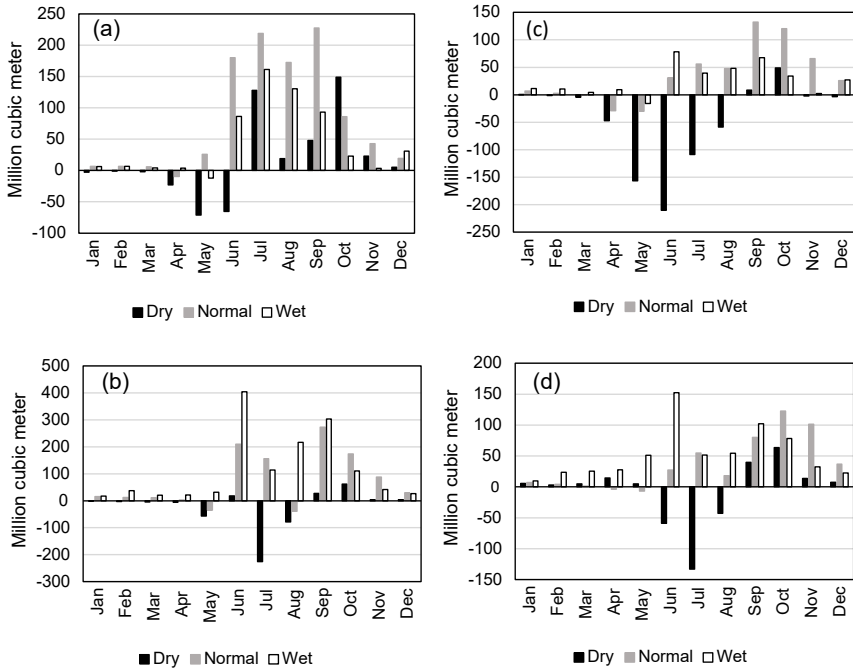
Figure 11.5. Left: Changes in average monthly flow at Monywa station during (a) 2015–2044 and (b) 2045–2074 under climate change scenarios. Right: Changes in average monthly groundwater flows at Monywa station during (c) 2015–2044 and (d) 2045–2074 under climate change scenarios
