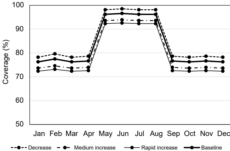
Figure 11.7. Domestic water coverage from different population scenarios for the Monywa sub-basin
