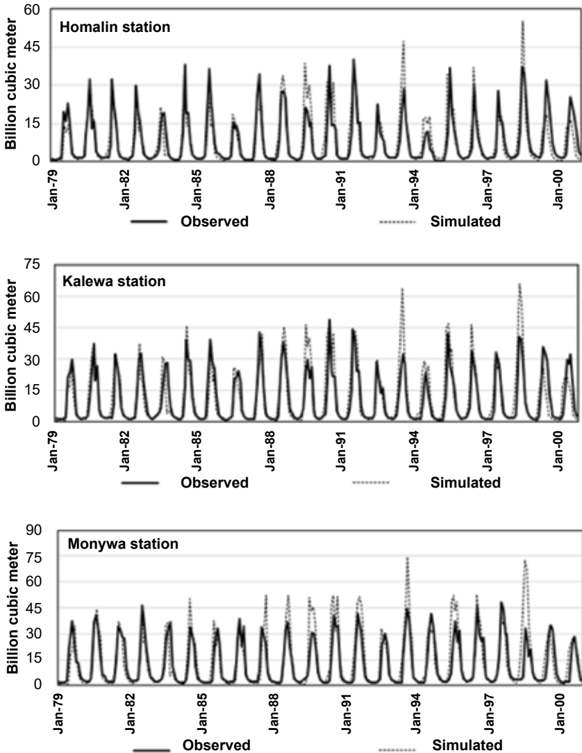
Figure 11.4. Monthly streamflow calibration (1979–2000) at three selected gauging stations on the Chindwin River
