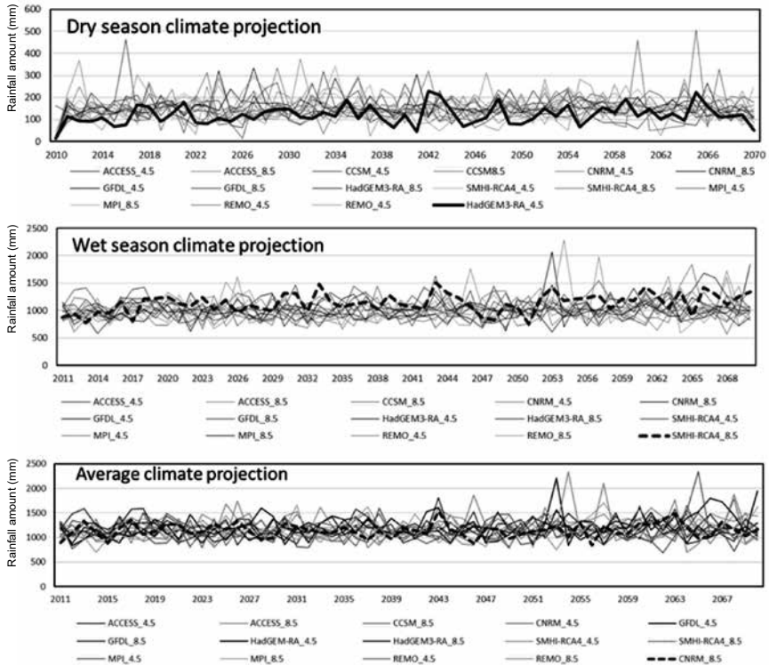
Figure 12.6. Projected average annual rainfall from eight Regional Climate Models (RCMs) under RCP 4.5 and 8.5 for normal, dry and wet climate model selection for the entire basin
