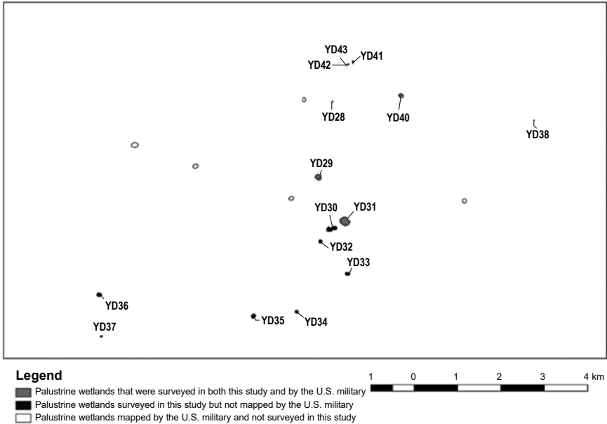
Figure 3.8. Palustrine wetlands located within Yok Don National Park, Vietnam, that were mapped by the US military (white with grey outlines), surveyed on the ground (black), or were evaluated by both efforts (grey). YD# refers to the wetland i.d. generated during the ground survey.
