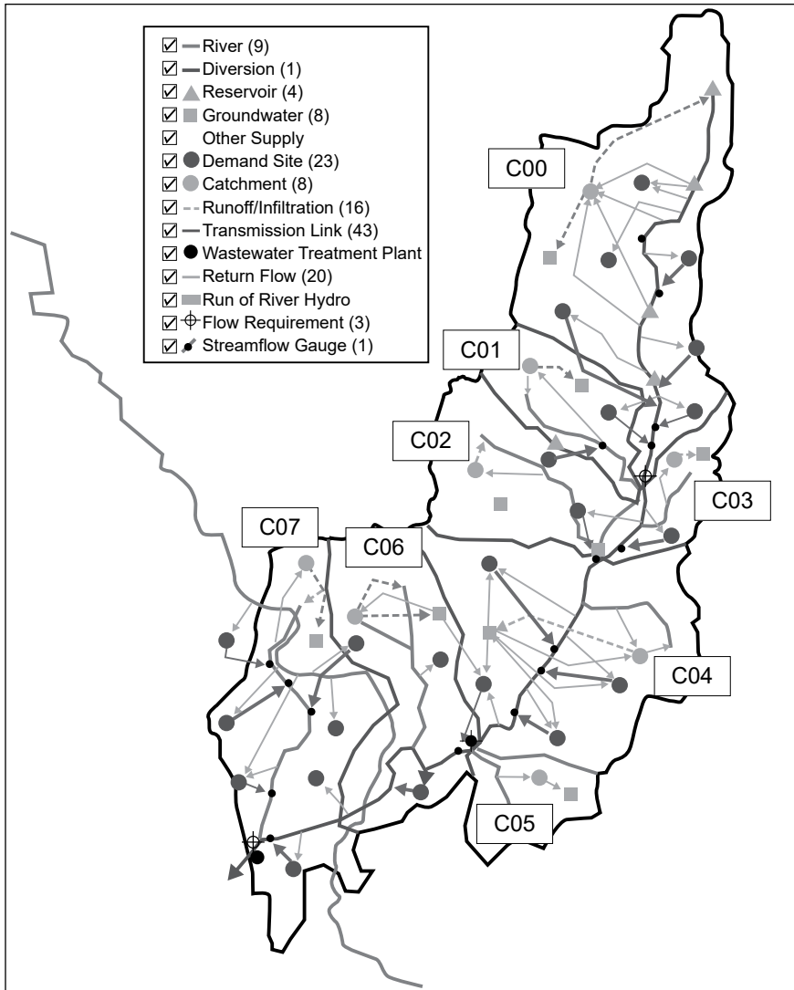
Figure 12.5. Water Evaluation And Planning (WEAP) model diagram of the Huay Sai Bat River Basin
