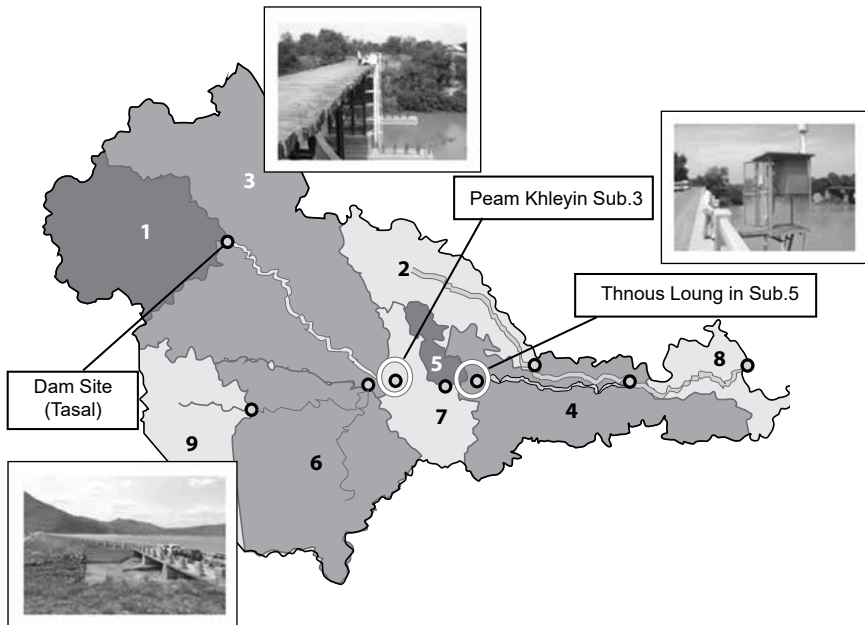
Figure 10.2. The delineated sub-catchment used in the SWAT model in the Prek Thnot River Basin
