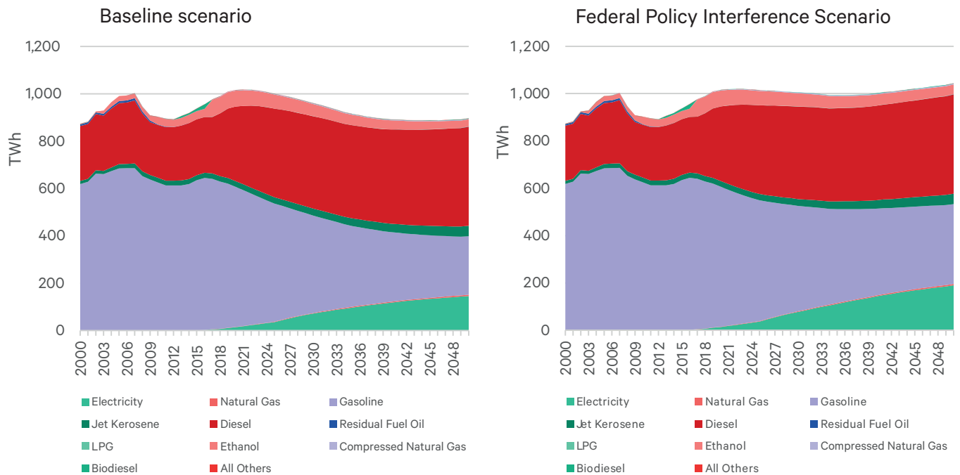
Figure 6: Comparison of transportation fuel demands in the baseline scenario (left) and Federal Policy Interference Scenario (right). Overall energy demands grow in the Federal Policy Interference Scenario.
