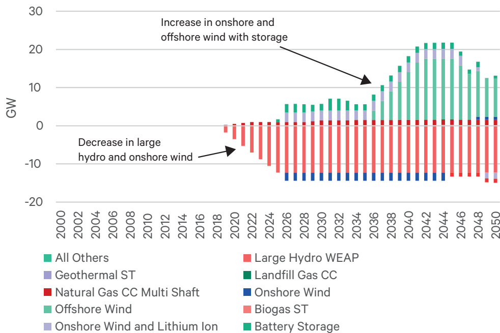
Figure 5: Difference in capacity between the Policy Baseline and No Hydropower Scenario
