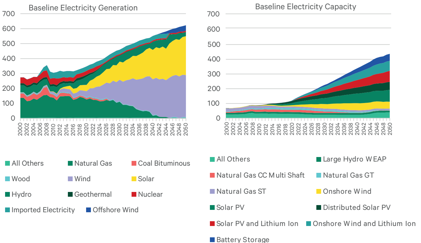
Figure 4: The left graph shows the make-up of electricity generation under a scenario where California implements existing policies (2050 = 623 TWH). The right graph shows the electricity capacity under the same scenario (2050 = 436 GW).
