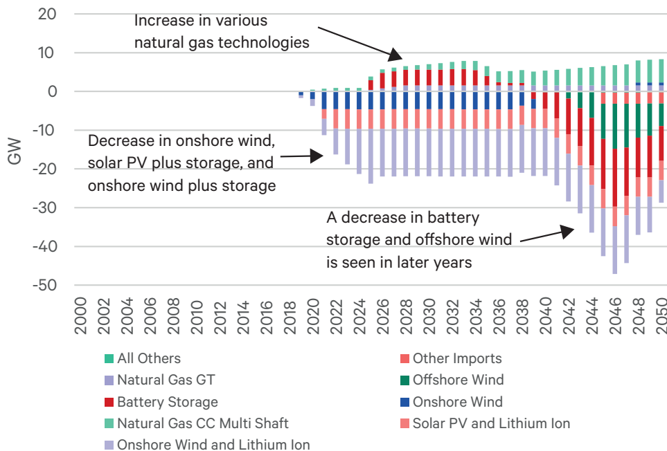
Figure 7: Difference in capacity between the Policy Baseline and Federal Policy Interference Scenarios.
